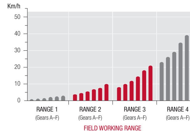
DYNA-6 TRANSMISSION
